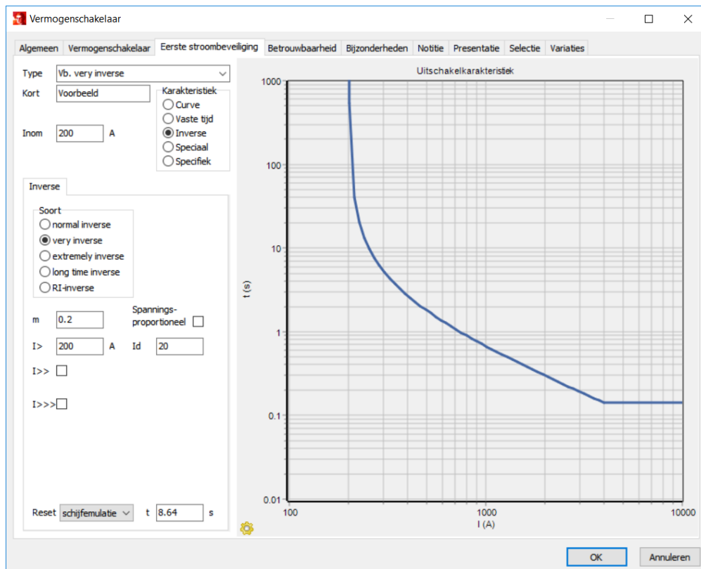
Figuur 7 Invoer AMT-relais in Vision Network Analysis
