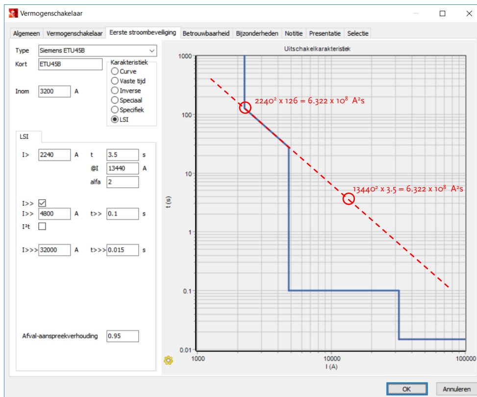
Figuur 32 LSI-beveiliging in Vision
