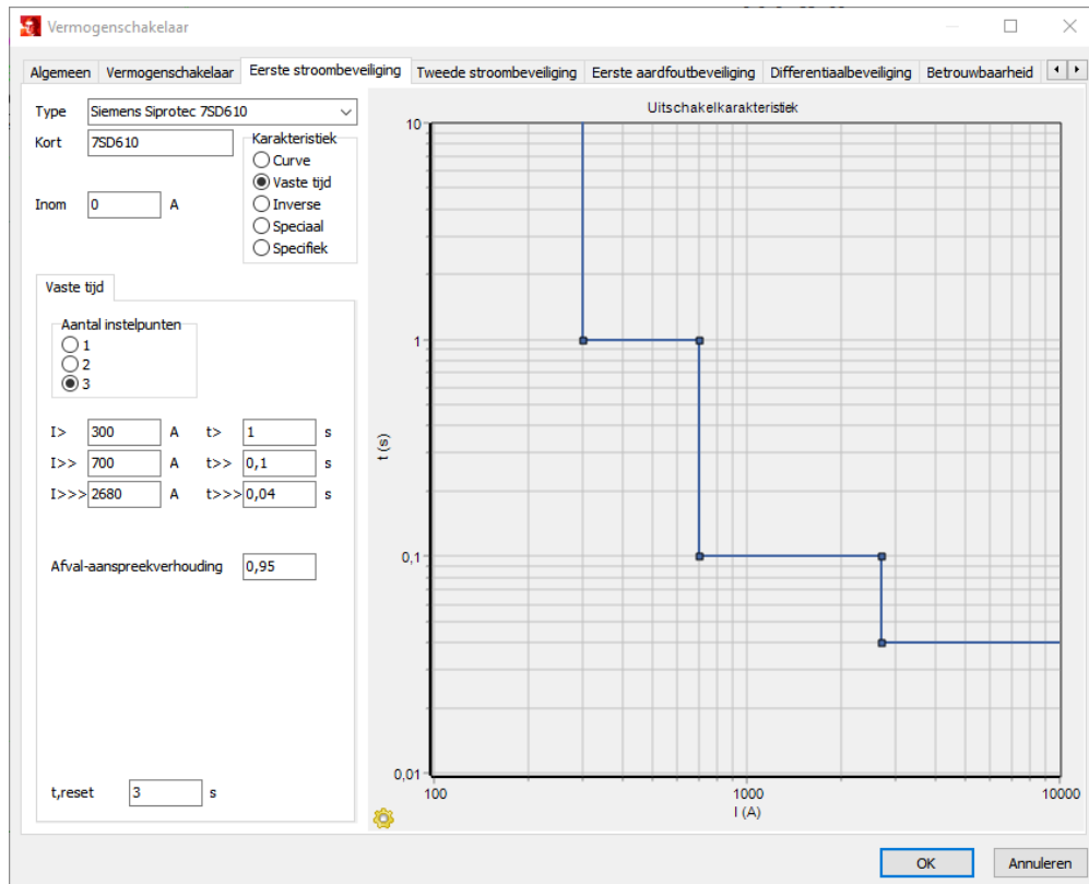
Figuur 13 Invoer OMT-relais in Vision Network Analysis
